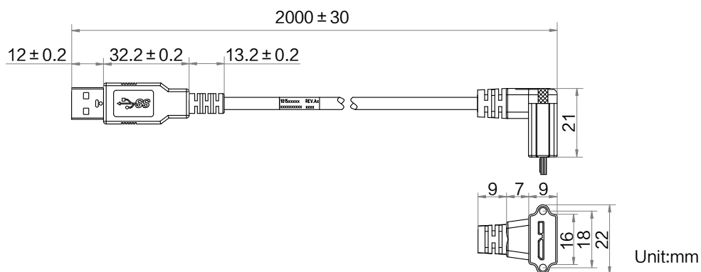
MV-ACU3-MBMs(down)-AM-ST-2m:
