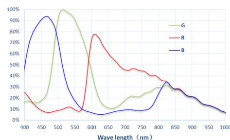
MV-CU013-80GC 响应曲线
