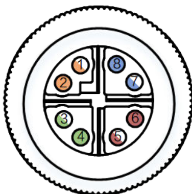
图 4-5 8-pin M12 X-Code
