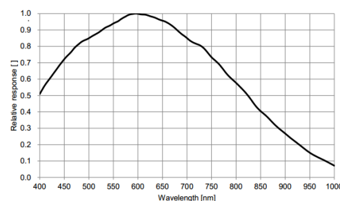
MV-CH120-10GM V5 量子效率
