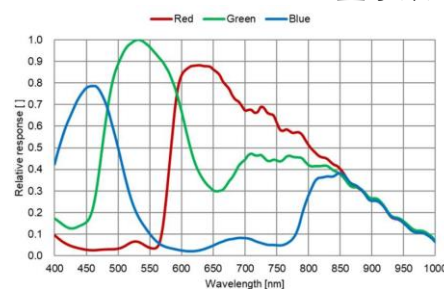
MV-CH123-10GC 量子效率
