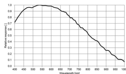
MV-CH123-10GM 量子效率
