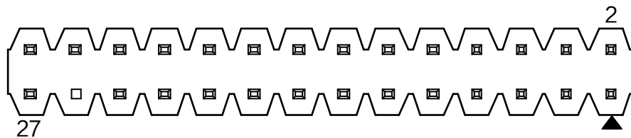
图4-2 27-pin 排针
