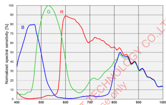
MV-CH610-10TC 量子效率
