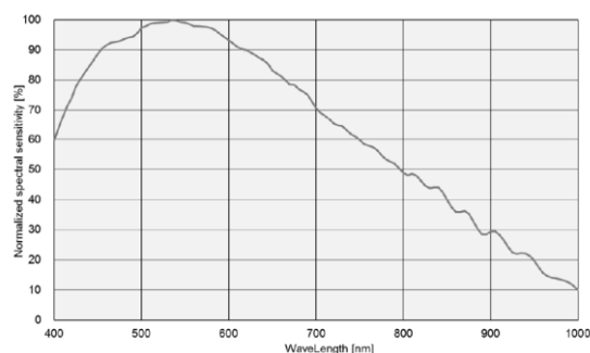
MV-CH610-10TM 量子效率
