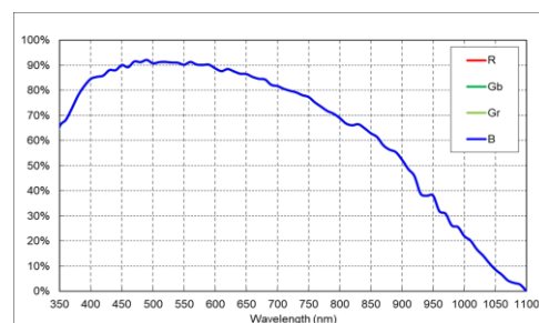
MV-CH120-60TM 量子效率
