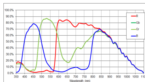
MV-CH120-60TC 量子效率
