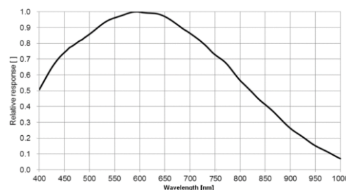
MV-CH050-10UM/UP 量子效率
