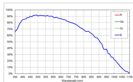
MV-CH089-60GM V5 量子效率
