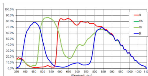
MV-CH089-60GC V5 量子效率
