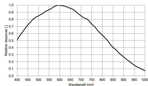
MV-CH120-10GM V4 量子效率
