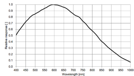
MV-CH120-10UM 量子效率
