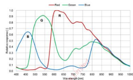
MV-CH120-10UC 量子效率
