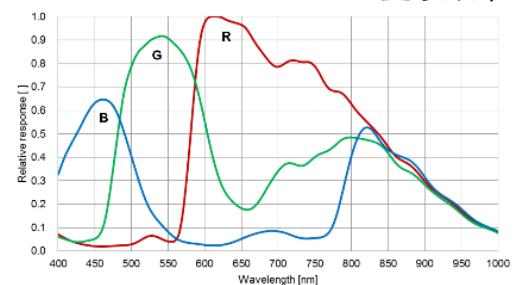
MV-CH120-10UC V5 量子效率
