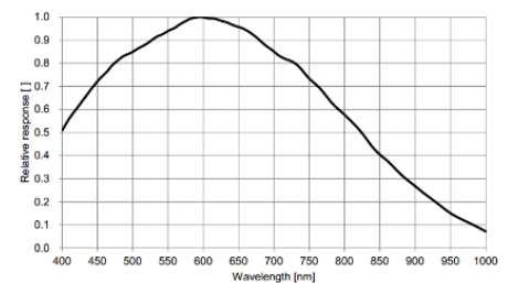
MV-CH120-10UM V5 量子效率
