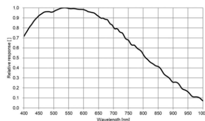
MV-CH123-10UM 量子效率
