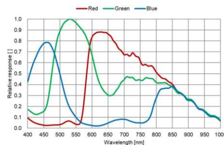
MV-CH123-10UC 量子效率
