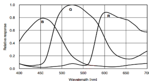
MV-CS120-10GC V5 响应曲线
