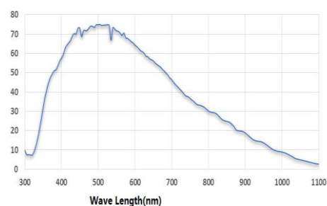
HK-YX31Z-2WM响应曲线
