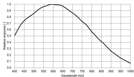
HK-YZ002-9WM量子效率
