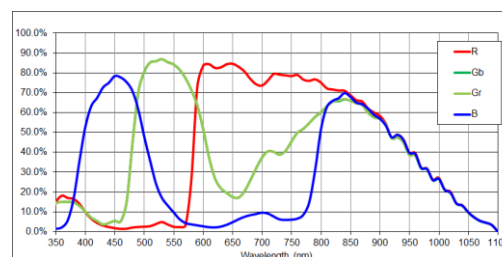
HIK-C120-CG 量子效率
