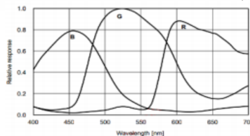
MV-XD0120-10GC 响应曲线
