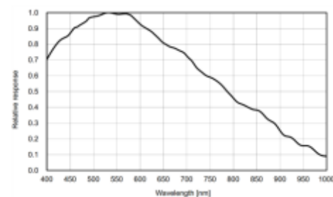
MV-XD0200-10UM V5 量子效率
