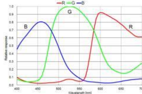
MV-XD6010GC V5 量子效率
