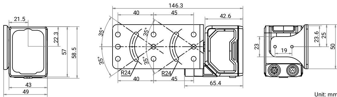
Installation Bracket:
