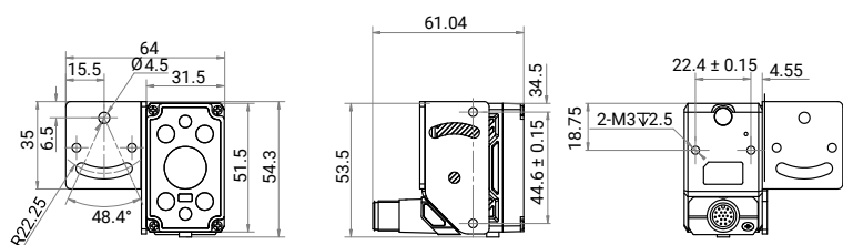
Device and Installation Bracket 1 (Right Angle)
