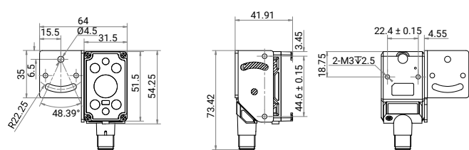
Device and Installation Bracket 2 (Straight Angle)
