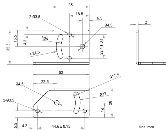
Bracket
