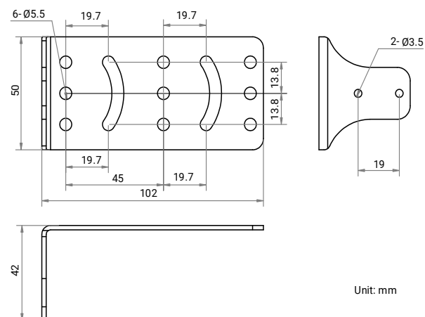
Installation Bracket:
