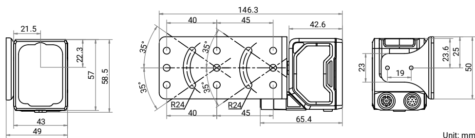
Installation Bracket:
